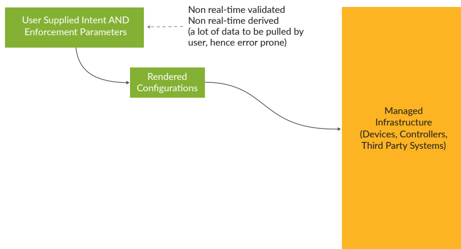
Figure 3: Typical stateless orchestration
