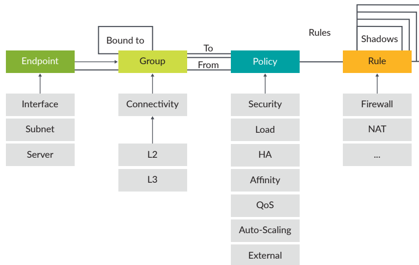
Figure 8: Group-based policies
