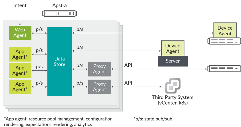
Figure 9: Apstra agents
